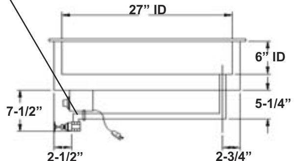
END VIEW
