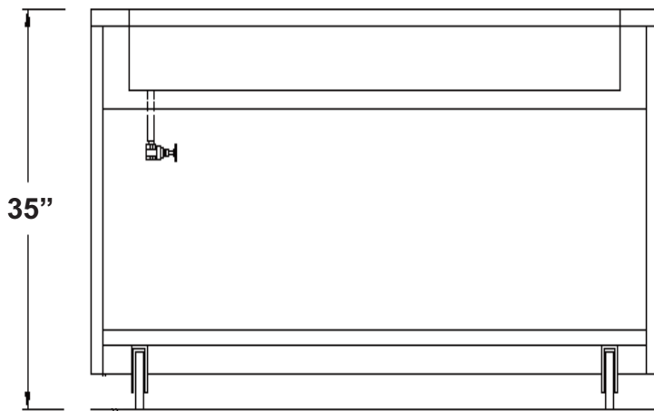
REAR ELEVATION
